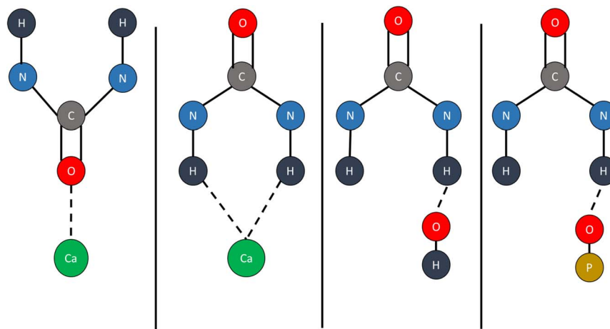
Fig. 4 Proposed bonding modes between \text{Ca}^{2+} , \text{O}_3\text{-PO}_3^- , and \text{OH}^- in HAP with –CO–, and NH– functional groups of urea. 35 Assignments were made based on previous literature reports using metal–urea complexes.
