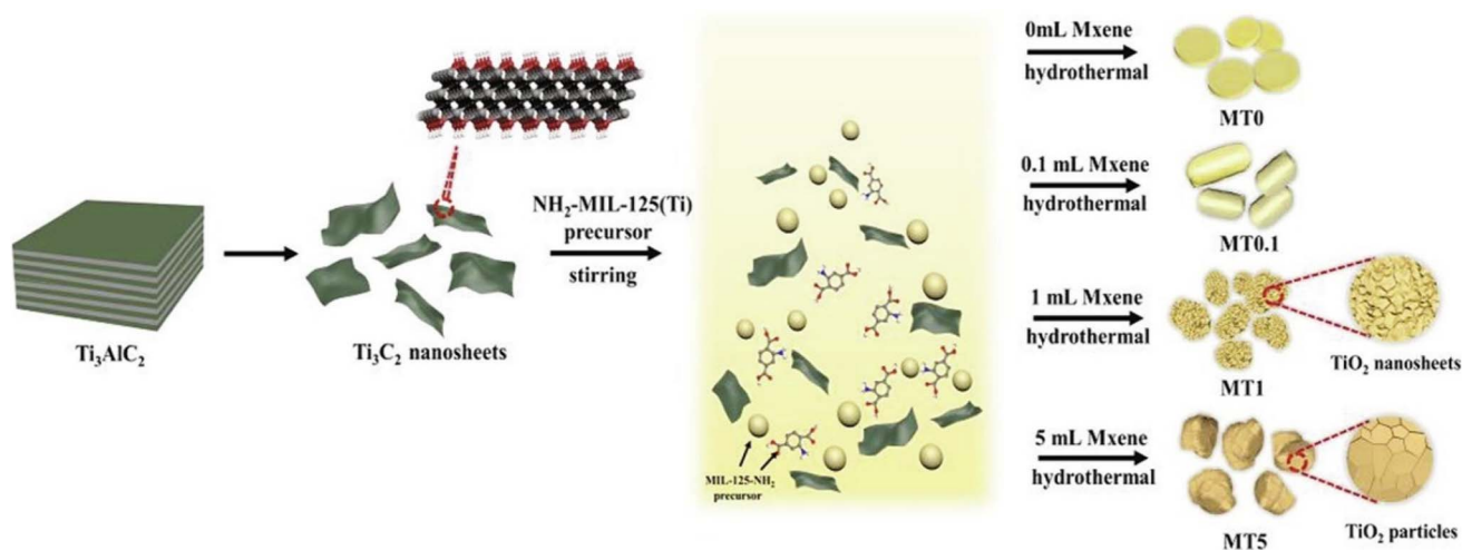
Fig. 5 Schematic of preparing Ti 3 C 2 nanosheets and MOFs-based heterostructure. Reproduced from ref. 55 with permission from Elsevier Ltd, copyright © 2020.
