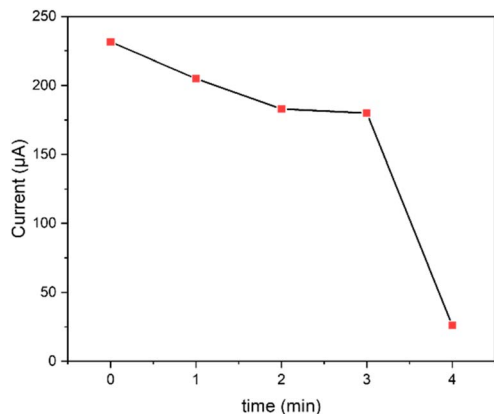
Fig. 9 Effect of accumulation time on the peak current of totalolone at the bio-NPs-ZnO/CPE electrode in 0.1 M NaCl solution (pH 4.5), at a scan rate of 100 mV s -1 and a start potential of -1.0 V vs. Hg/Hg 2 Cl 2 , KCl sat.
