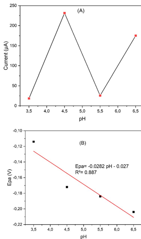
Fig. 8 (A) Influence of solution pH on the oxidation peak current of totarolone recorded at bio-ZnO-NPs-ZnO/CPE in 0.1 M NaCl, at a scan rate of 100 mV s −1 and a start potential of −1.0 V vs. Hg/Hg 2 Cl 2 , KCl sat. and (B) linear plot of E_{pa} vs. pH.
