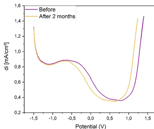
Fig. 13 Bio-NPs-ZnO/CPE stability; amplitude: 20 mV; potential step: 5 mV; start potential: -1.5 V vs. Hg/Hg 2 Cl 2 , KCl sat.
