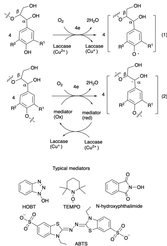
Fig. 3 Laccase-mediated oxidation. 17,29,76–78
