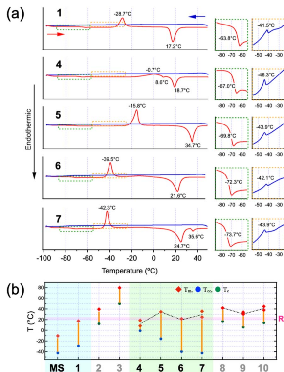
Fig. 2 (a) DSC thermograms of liquid samples ( 1, 4, 5, 6 and 7 ). All samples were first heated from RT to 50\text{ }^{\circ}\text{C} , and then subjected to cooling and reheating at a rate of 10\text{ }^{\circ}\text{C min}^{-1} . The cooling and heating processes are represented by blue and red lines, respectively. The regions with weak signals (highlighted by green and orange dotted lines) are enlarged and displayed on the right side. (b) Graphical representation of the thermal data presented in Table S1, SI.
