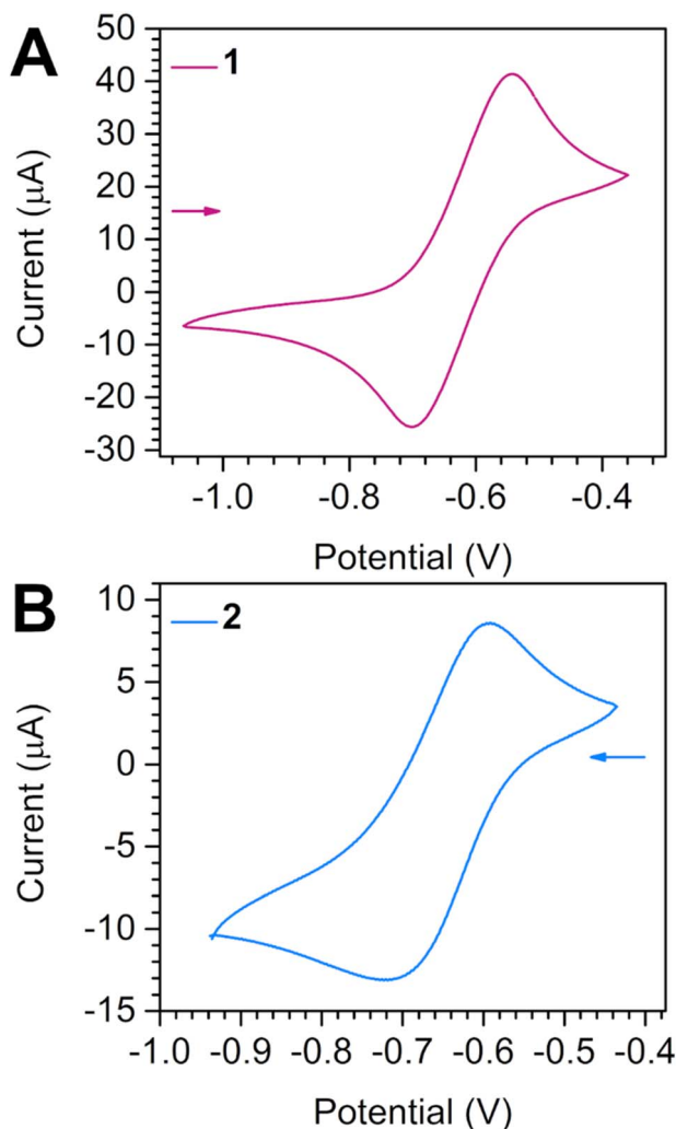
Fig. 3 Cyclic voltammograms of [(Cp^*_2Dy)_2(\mu-tan)] (1) (A) and [(Cp^*_2Dy)_2(\mu-tan')][BARF_{20}] (2) (B), measured in DCM at 300 K with 0.22 \text{ mmol L}^{-1} [^nBu_4N][PF_6] supporting electrolyte and 3 \text{ mmol L}^{-1} analyte concentration against a Ag wire pseudo reference electrode with a 100 \text{ mV s}^{-1} scan rate.
