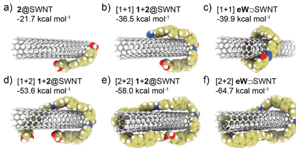
Fig. 6 Local minima and \Delta G_a values in \text{kcal mol}^{-1} computed at the \omega\text{B97X-3c/SMD}(\text{H}_2\text{O})//\text{GFN2/ALPB}(\text{H}_2\text{O}) level of theory, 16,17,22,23 for the potential aggregates formed by the association between a truncated hydrogen-capped section of a (6,5)-SWNT (ball-and-stick), and cyclic (c and f)/oligomeric (a, b, d and e) species arisen from the self-assembly of building blocks 1 and 2 (van der Waals spheres).
