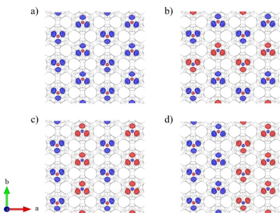
Fig. 2 Spin density of considered magnetic configurations for V_3N@C_{80} . (a) Ferromagnetic (FM), (b) zig-zag, (c) single-stripe and (d) double-stripe antiferromagnetic (AFM) configurations. Color code: spin up (blue) and down (red) electrons.
