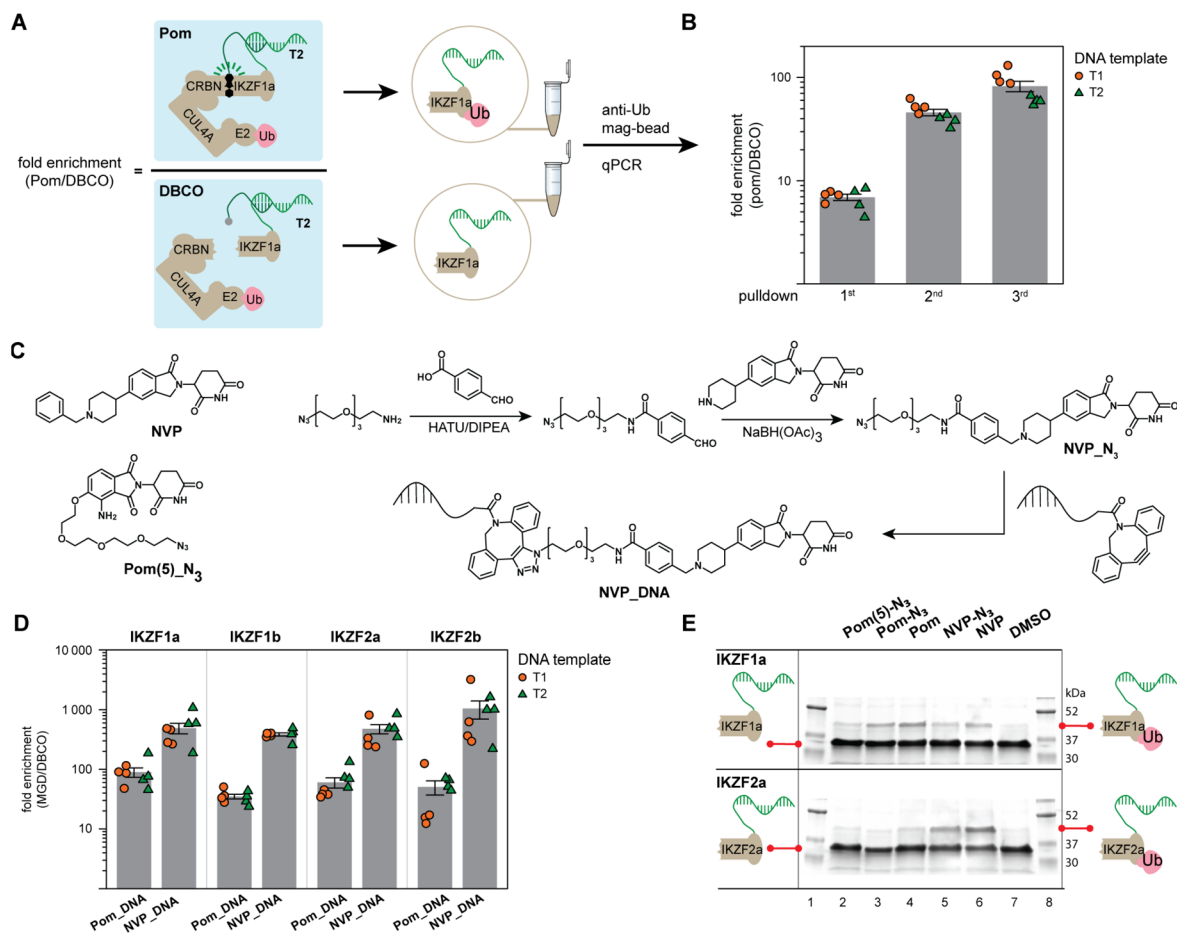
Fig. 4 Establishing the enrichment assay. (A) Pom DNA and DBC O DNA were independently tested for Ub-transfer to a partially complementary template DNA bearing IKZF1a ( IKZF1a DNA ). (B) Fold enrichment of Pom DNA versus DBC O DNA over three consecutive pull-downs using anti-Ub magnetic beads; different templates were tested (T1 and T2) to generate the data to insure that qPCR bias does not impact the enrichments (for absolute DNA quantitation by qPCR, as well as details on the pull-down conditions and optimization of the protocol, see ESI Section 8†). (C) Structures of Pom(5) N 3 and NVP , as well as synthesis of NVP N 3 and NVP DNA . (D) In vitro ubiquitination of IKZFs with Pom DNA and NVP DNA expressed as fold enrichment (relative to DBC O-bearing DNA) after anti-Ub magnetic beads purification and qPCR. (E) In vitro ubiquitination of MGDs with and without linkers to examine the effect of linker on Ub-transfer efficiency. MGD = molecular glue degrader.
