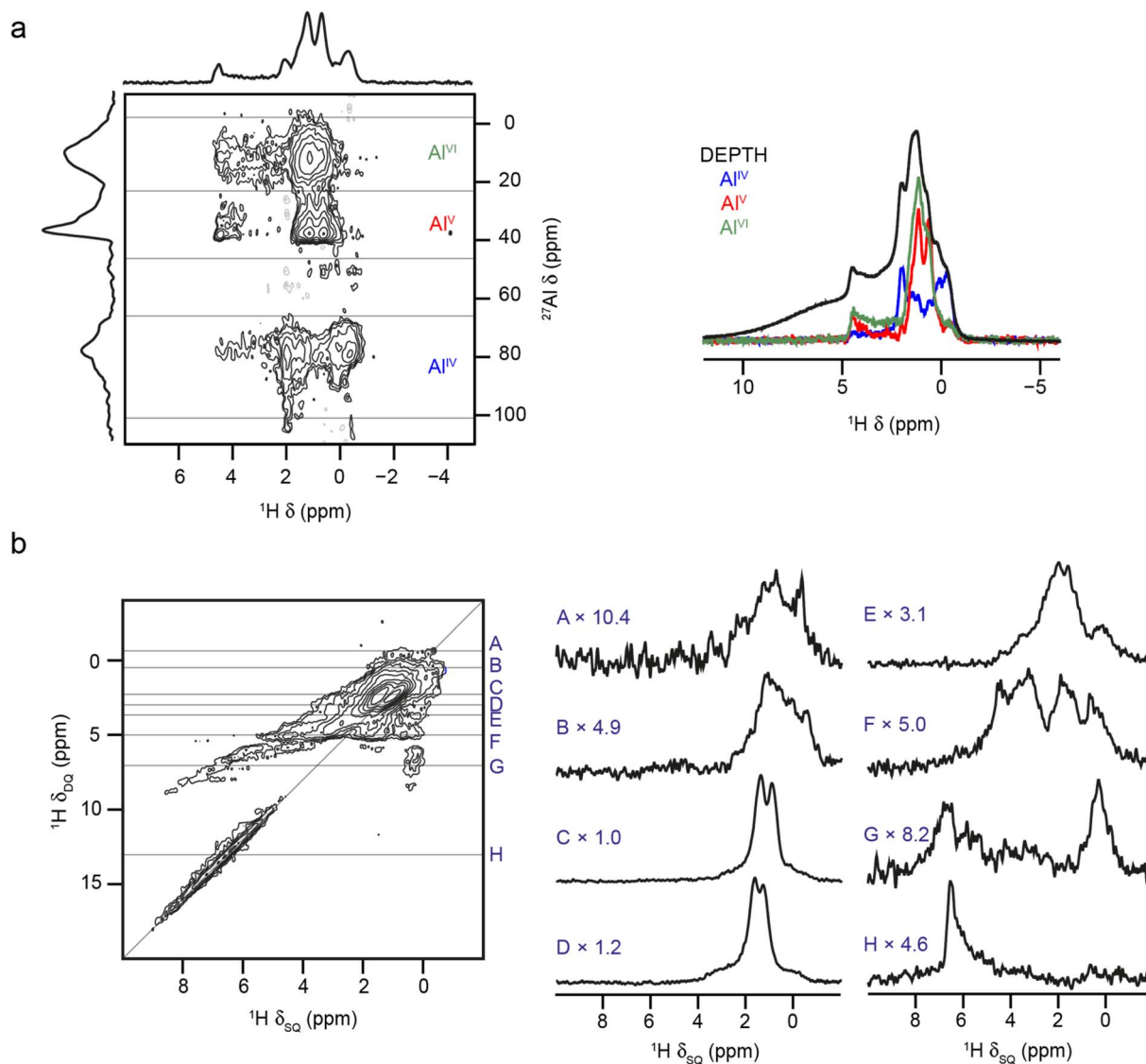
Fig. 11 (a) {}^1\text{H} - {}^{27}\text{Al} (14.1 T, 40 kHz) D-HMQC spectrum (with TRAPDOR recoupling) of \gamma\text{-Al}_2\text{O}_3 dehydrated at 550 ^\circ\text{C} , with sum projections (extracted parallel to \delta_2 ) over the regions corresponding to \text{Al}^{\text{IV}} , \text{Al}^{\text{V}} and \text{Al}^{\text{VI}} (as shown), overlaid with the {}^1\text{H} DEPTH (14.1 T, 40 kHz) DEPTH MAS NMR spectrum of \gamma\text{-Al}_2\text{O}_3 dehydrated at 550 ^\circ\text{C} . (b) {}^1\text{H} (14.1 T, 40 kHz) DQ MAS spectrum (acquired using BABA recoupling) of \gamma\text{-Al}_2\text{O}_3 dehydrated at 550 ^\circ\text{C} , with cross sections (extracted parallel to \delta_2 and vertically expanded as shown) extracted at the \delta_1 positions indicated. For detailed experimental parameters see Section S1 of the ESI.†
