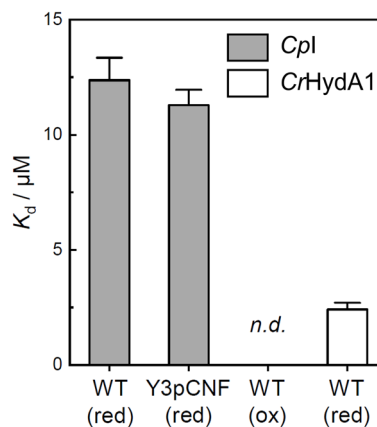
Fig. 6 Microscale thermophoresis. Dissociation constants ( K_d ) of the CpFd : CpI (WT) and Y3pCNF- CpFd : CpI complex under reducing or oxidizing conditions (red/ox). Under oxidizing conditions in the absence of dithionite, an interaction between CpFd : CpI was not detected (n.d.). The open bar depicts the K_d of the CpFd : CrHydA1 complex under reducing conditions. See Fig. S7† for the titration curves and additional data.
