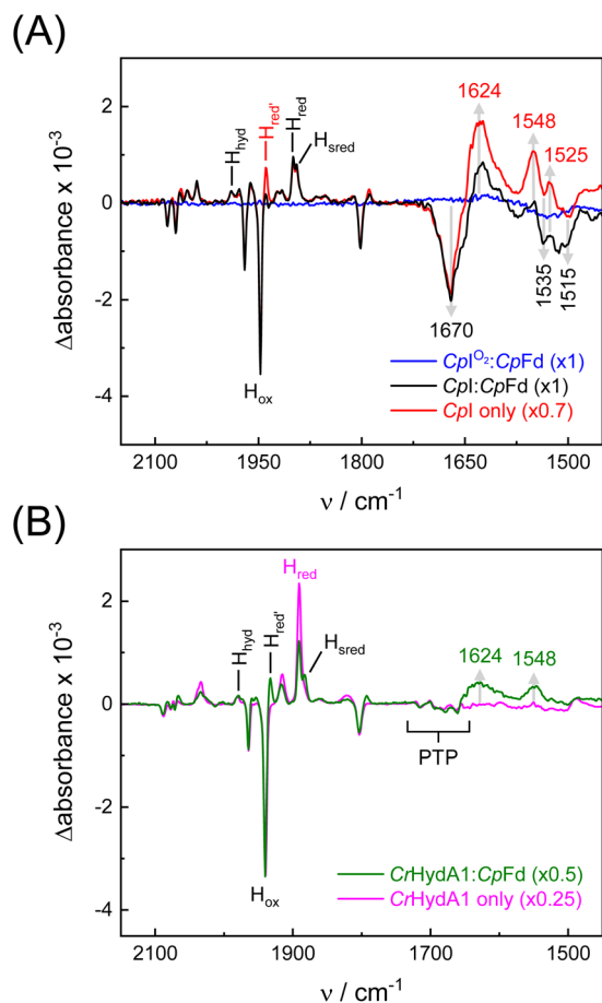
Fig. 5 Infrared difference spectroscopy. (A) \text{H}_2\text{-N}_2 ATR FTIR difference spectra of Y3pCNF- CpFd : CpI (black) and CpI alone (red) after 25 s. Bands above 1750\text{ cm}^{-1} are assigned to H-cluster ligands in the H_{\text{ox}} state (negative) and various reduced states (positive). At lower frequencies, the 1670/1624\text{ cm}^{-1} down-shift in the amide I regime indicates protein structural changes, alongside up-shifts at 1535/1548\text{ cm}^{-1} and 1515/1525\text{ cm}^{-1} . The blue spectrum serves as a negative reference where CpI was inactivated with \text{O}_2 ahead of the reaction with \text{H}_2 . (B) \text{H}_2\text{-N}_2 ATR FTIR difference spectra of Y3pCNF- CpFd : CrHydA1 (green) and CrHydA1 alone (magenta) after 50 s. Note the lack of the difference features in CrHydA1 in the amide I regime while only small changes are observed in the presence of Y3pCNF- CpFd . "PTP" refers to small difference features explored earlier. 62 All spectra are normalized to the main CO band of H_{\text{ox}} ( 1947\text{ cm}^{-1} in CpI , 1940\text{ cm}^{-1} in CrHydA1 ) with factors as indicated in the legends.
