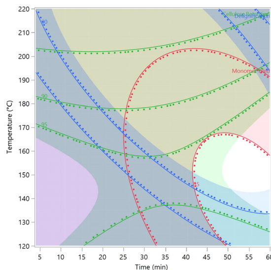
Fig. 12 Contour profiler of the optimum reaction conditions when longer reaction time is preferred. Reaction conditions: T = 140\text{--}160\text{ }^{\circ}\text{C} , t = 50\text{--}60\text{ min} , \text{O}_2\text{ (psi)} = 40\text{ psi} , catalyst = 0 mg, NaOH = 1.43 M, yield >35 wt%, glucan retention >97 wt%, delignification = 95 wt%.
