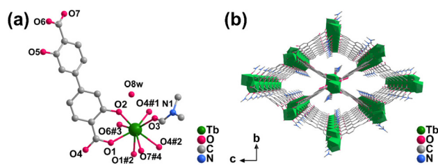
Fig. 1 (a) The asymmetric unit of Tb-MOF-1 . (b) The 3D frame aggregation along the a -axis of Tb-MOF-1 . All hydrogen atoms and free water molecules are omitted for clarity. Symmetry codes: #1 1 + x, y, z ; #2 1 - x, -y, 1 - z ; #3 1 - x, -1/2 + y, 1/2 - z ; #4 x, 1/2 - y, 1/2 + z .
