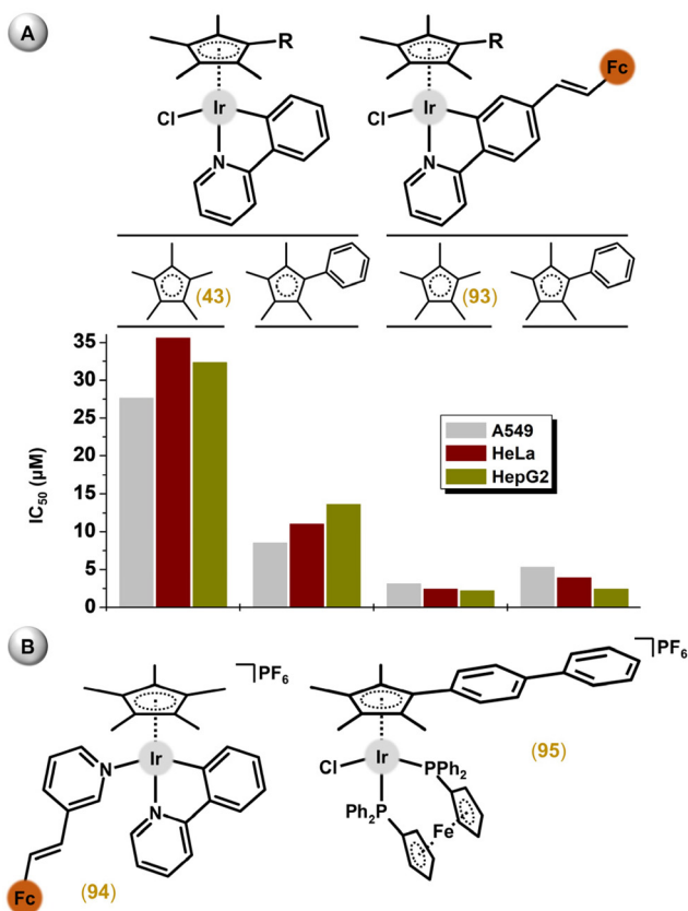
Fig. 23 (A) Structural formulas and in vitro antiproliferative activity of [Ir( \eta^5 -Cp x )Cl(ppy FC )] complexes 43 and 93 , containing various Cp x derivatives (Cp* or Cp Ph ) in combination with ppy or its ferrocene (Fc)-substituted derivative (ppy FC ). (B) Structural formulas of ferrocene-containing complexes 94 and 95 .
