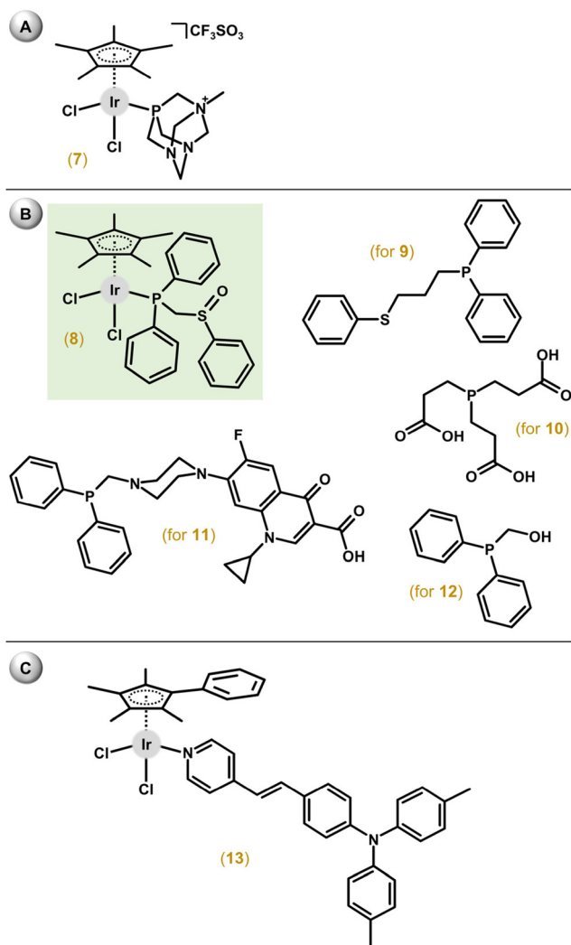
Fig. 4 Structural formulas of (A) ionic complex [\text{Ir}(\eta^5\text{-Cp}^*)\text{Cl}_2(\text{mpta}^+)] \text{CF}_3\text{SO}_3 ( 7 ), (B) electroneutral complex [\text{Ir}(\eta^5\text{-Cp}^*)\text{Cl}_2(\text{phs}^1)] ( 8 ) and P-donor ligands \text{phs}^2 , tcep, psf and poh involved in analogues 9–12 , respectively, and (C) complex 13 with monodentate N-donor ligand from (B).
