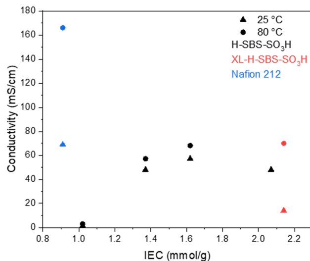
Fig. 8 Conductivity at 25^\circ\text{C} (circle) and 80^\circ\text{C} (triangle) of H-SBS- \text{SO}_3\text{H} (black), XL-H-SBS- \text{SO}_3\text{H} -2.14 (red) and Nafion 212 (blue).
