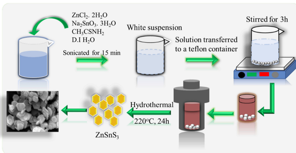
Scheme 1 Synthesis process scheme for LN-ZnSn 3 nanocrystals.
