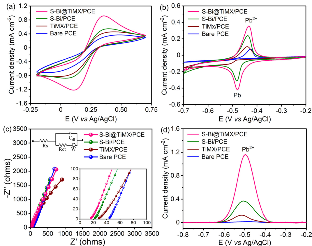
Fig. 6 CVs of bare PCE, TiMX/PCE, S-Bi/PCE, and S-Bi@TiMX/PCE at 50 \text{ mV s}^{-1} in (a) 5.0 mM ( K_4[Fe(CN)_6] ) solution with 0.1 M KCl, (b) 0.08 M HClO_4 containing 10 \text{ mg L}^{-1} Pb^{2+} , (c) EIS, and (d) SWASV responses of bare PCE, TiMX/PCE, S-Bi/PCE, and S-Bi@TiMX/PCE in 0.08 M HClO_4 solution containing 50 \text{ µg L}^{-1} Pb^{2+} .
