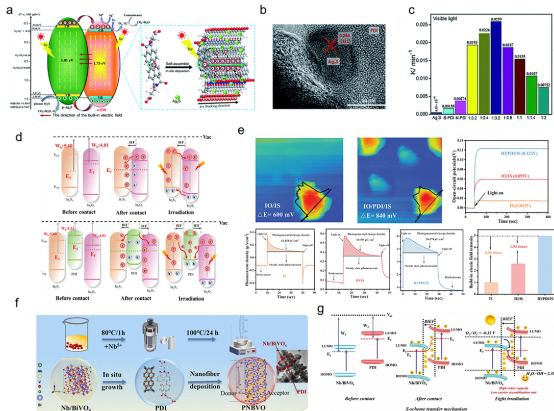
Fig. 11 (a) Mechanism of Ag 2 S/PDI. (b) The HR-TEM image of Ag 2 S/PDI (1:0.6). (c) Visible light irradiation (where B-PDI represents bulk-PDI, N-PDI represents nano-PDI, and 1:1 represents the mass ratio of Ag 2 S to PDI). Reproduced from ref. 104. Copyright 2019, the Royal Society of Chemistry. (d) Schematic illustration of the charge migration between IO/IS and IO/PDI/IS. (e) The calculation of IEF intensity of IS, IO/IS and IO/PDI/IS. Reproduced from ref. 105. Copyright 2023, Wiley. (f) Schematic illustration of the facile solvothermal preparation of PNBVO composite materials. (g) Photocatalytic electron transfer mechanism of PNBVO. Reproduced from ref. 106. Copyright 2025, Elsevier.
