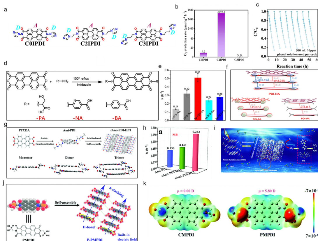
Fig. 2 (a) Different \sigma lengths of molecular structures about CnIPDI. (b) Comparison of photocatalytic \text{O}_2 evolution rate on CnIPDI. (c) Cyclic stability of C2IPDI. Reproduced from ref. 56. Copyright 2023, Wiley. (d) The synthesis method of PDI-NA molecular and reference catalyst. (e) TOC removal rate and mineralization rate constant over different photocatalysts. (f) A schematic diagram of PDI-NA, PDI-BA and PDI-PA. Reproduced from ref. 33. Copyright 2022, Elsevier. (g) The synthesis process and structure of sAmi-PDI-HCl (over) and the DFT calculations regarding geometries of sAmi-PDI-HCl monomers, dimers, and trimers (below). (h) The kinetics constants toward MB. (i) The mechanism for the photocatalytic degradation process when using amide-functionalized supramolecular PDI. Reproduced from ref. 30 Copyright 2020, the Royal Society of Chemistry. (j) The synthesis of supramolecular P-MPDI. (k) Diagram of molecular dipoles and electron distribution in PDI derivatives. Reproduced from ref. 62. Copyright 2019, the Royal Society of Chemistry.
