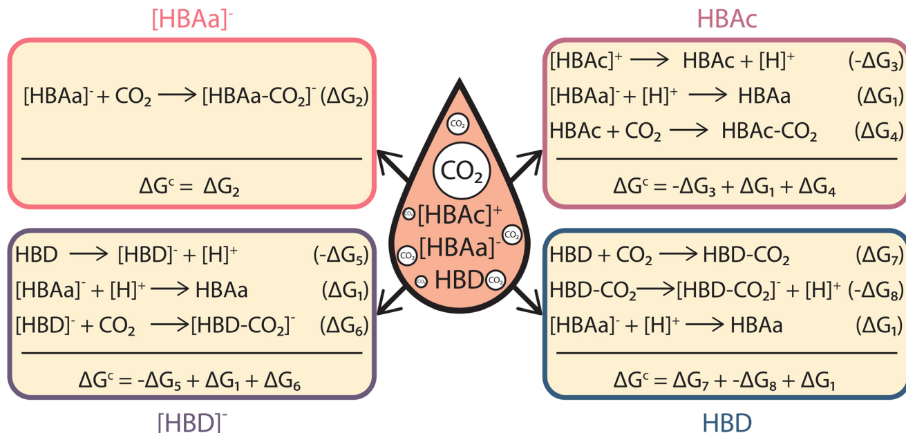
Fig. 3 The different CO 2 complexation pathways considered for a [HBAA] + [HBAa] - :HBD ES. Complexation occurs via the [HBAa] - (pink), HBAAc (mauve), [HBD] - (purple), and HBD (blue) pathways. Reaction numbers are the same as in Table 1. Only the [HBAa] - pathway does not require a proton transfer for CO 2 complexation. The other three pathways all involve an intermolecular proton transfer, which is modeled here as occurring to the [HBAa] - species.
