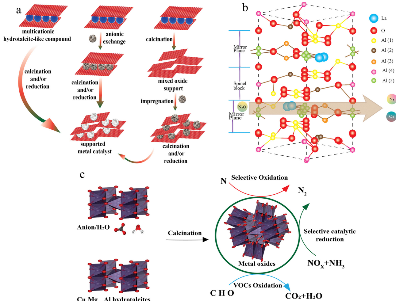
Fig. 9 (a) Representation of main routes leading to the synthesis of metal-supported catalysts from LDH precursors. 139 Reproduced with permission from Springer (Copyright©2003). (b) \text{N}_2\text{O} decomposition to \text{N}_2 and \text{O}_2 in the mirror plane phase of perovskite-type La-hexaaluminates ( \text{LaFe}_x\text{-Al}_{12-x}\text{O}_{19} ). 140 Reproduced with permission from the American Chemical Society (Copyright©2014). (c) Hydroxalate-derived \text{Cu}_x\text{Mg}_{3-x}\text{AlO} oxides for pollutant-destruction mechanism. 141 Reproduced with permission from the American Chemical Society (Copyright©2019).
