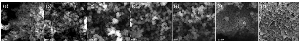
Fig. 3 SEM images of PDA NPs, after 24 h, at different \text{NH}_4\text{OH} percentage; (a) 0.056%, (b) 0.11%, (c) 0.22%, (d) 0.45%, (e) 0.89%, (f) 1.79%, and (g) 3.58%.
