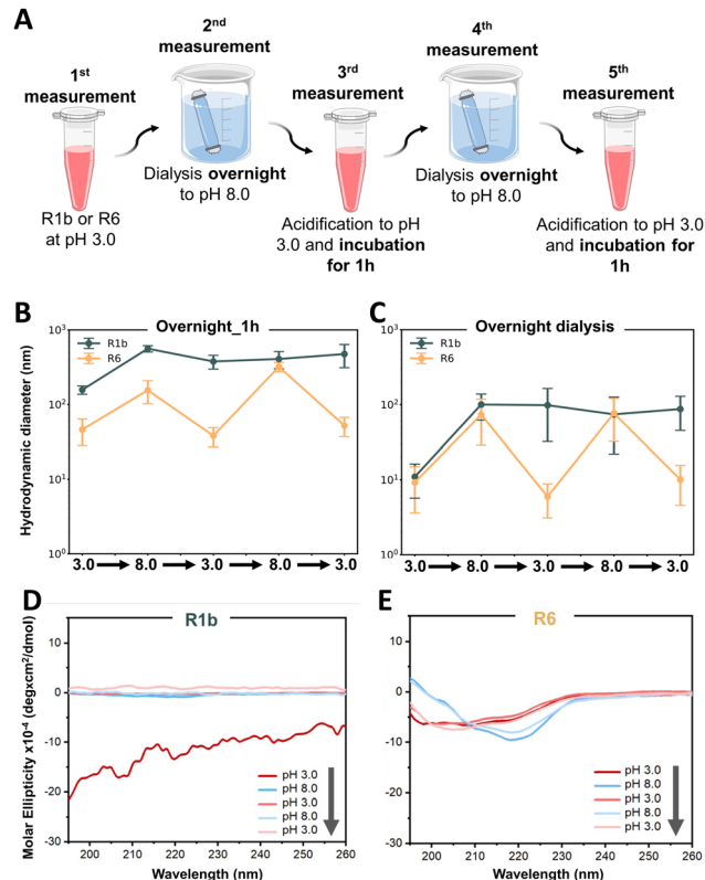
Fig. 5 Reversibility of reflectin self-assembly under cyclic pH treatments. (A) Schematic representation of the experimental strategy. Protein samples were subjected to alternating pH conditions (3.0 and 8.0) and analysed at each stage. Overnight dialysis was used for pH transitions to 8.0, while acidification to pH 3.0 was followed by 1h incubation. (B) DLS measurements of hydrodynamic diameter for R1b and R6 with 1 h incubation after acidification and (C) with overnight dialysis for all pH transitions. Data points represent the mean value of measured hydrodynamic diameter \pm standard deviation of triplicate measurements for each sample. (D)–(E) Far-UV circular dichroism (CD) spectra monitoring conformational changes of R1b (D) and R6 (E) throughout pH cycles. The grey arrow indicates the sequence of pH variations.
