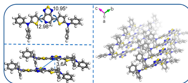
Fig. 5 Single-crystal structure of the compound DTPTS-PT. Reprinted (adapted) with permission from ref. 52. Copyright 2019 American Chemical Society.
