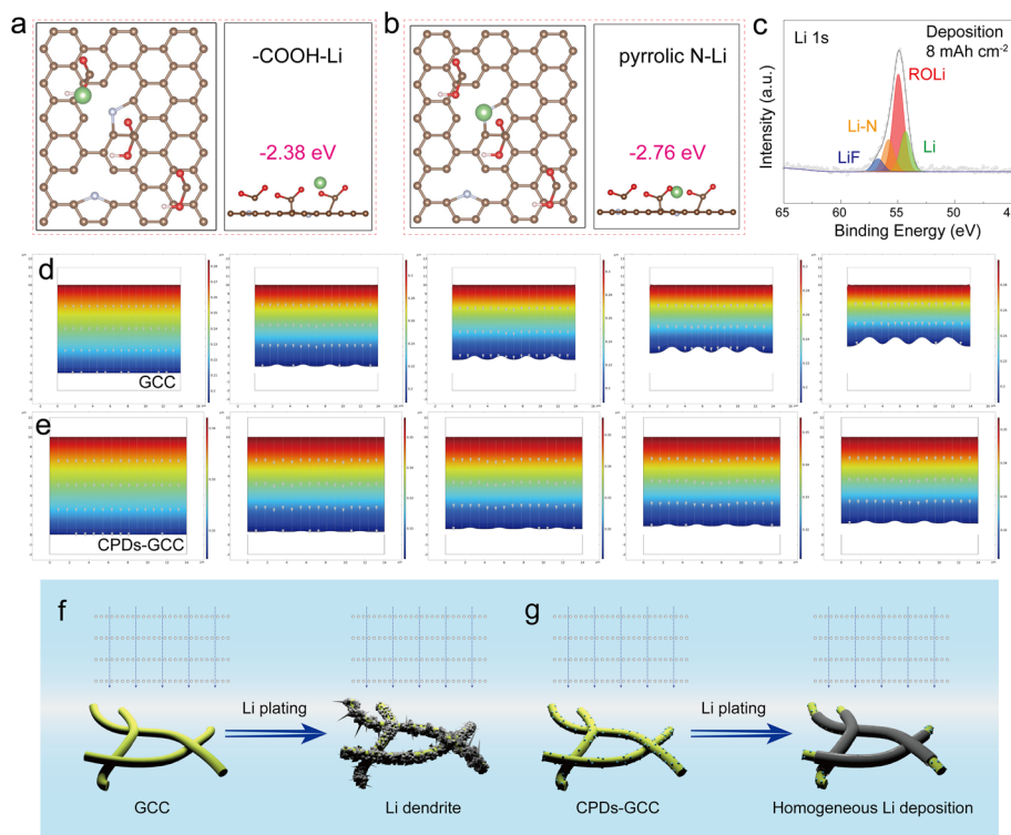
Fig. 3 Schematics of the model for bonding energy calculation between Li and different functional group atoms, and its corresponding Li adsorption energies. (a) -\text{COOH}-\text{Li} and (b) pyrrolic \text{N}-\text{Li} . (c) XPS spectrum of Li 1s for the CPD-GCC anode after Li deposition. Simulated ion concentration distributions during the process of Li deposition on different anodes: (d) GCC and (e) CPD-GCC anodes. (f and g) Illustration of Li plating on the GCC and CPD-GCC anodes.
