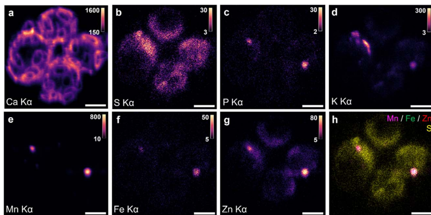
Fig. 2 Nano-XRF analysis of dried, coccolith-bearing G. huxleyi showing (a) Ca K\alpha XRF, (b) S K\alpha XRF, (c) P K\alpha XRF, (d) K K\alpha XRF, (e) Mn K\alpha XRF, (f) Fe K\alpha XRF, and (g) Zn K\alpha XRF maps. (h) Composite map of Mn, Fe, Zn, and S XRF signals. Intensity scale shown as XRF counts. Scale bar 2 \mu\text{m} .
