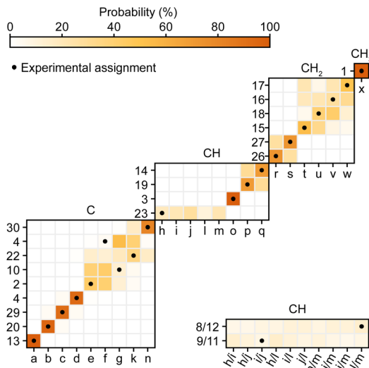
Fig. 12 Marginal individual assignment probabilities of ^{13}\text{C} chemical shifts of Atuliflapron obtained using correlated ^1\text{H} - ^{13}\text{C} chemical shift distributions and spectral editing. 244 For the probability map, labels along the vertical axis indicate nuclei (according to the inset in Fig. 11), and labels along the horizontal axis denote experimental shifts labelled alphabetically in order of decreasing ^{13}\text{C} shift. The carbon multiplicity is indicated above each marginal assignment probability map. Adapted from ref. 244.
