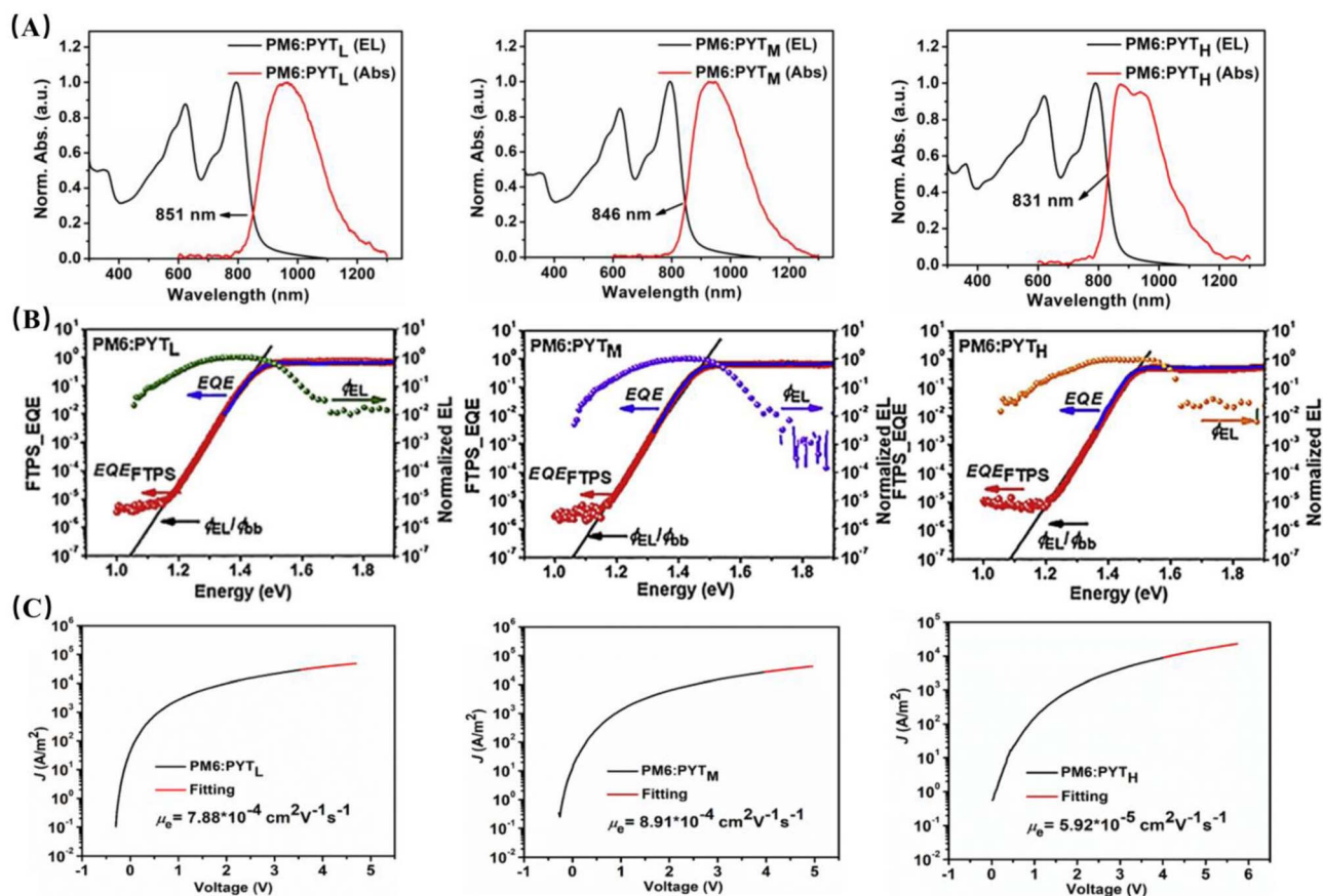
Fig. 2 (A) Normalized absorption and EL spectra of PM6:PYT L , PM6:PYT M , and PM6:PYT H blends; (B) semi-logarithmic plots display the normalized electroluminescence (EL), the measured external quantum efficiency (EQE), and the EQE derived from Fourier-transform photocurrent spectroscopy (EQE FTSPS ) as functions of photon energy for devices based on PM6:PYT L , PM6:PYT M , and PM6:PYT H ; (C) the dark J-V characteristics of PM6:PYT L , PM6:PYT M , and PM6:PYT H based electron-only devices. The red lines represent the best fitting using the SCLC model. Copyright 2020 Elsevier.
