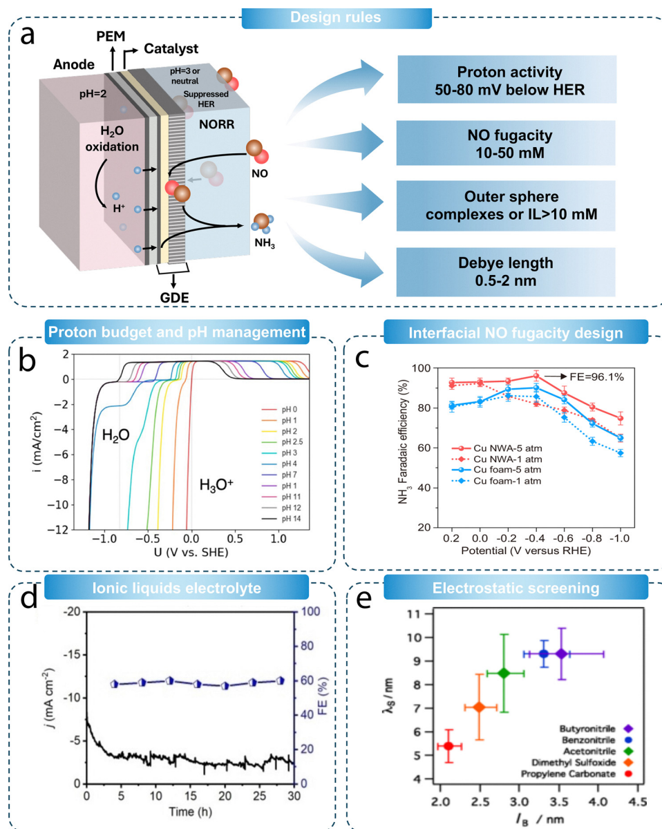
Fig. 5 (a) Design of electrochemical interfaces for efficient NORR. (b) Computed HER/HOR polarization curves using the DFT activation energies and mean-field microkinetic modeling. 113 Copyright 2019, American Chemical Society. (c) \text{NH}_3 FE over Cu NWA and commercial Cu foam at different applied potentials at 25 °C under 1 atm, 5 atm NO, respectively. 112 Copyright 2025, Springer Nature. (d) Chronoamperometry stability test of P-MoS 2 /NS in NO-saturated IL electrolyte at -0.7 V vs. RHE. 123 Copyright 2022, Wiley-VCH. (e) The measured electrolyte screening lengths are consistent with a linear increase with the Bjerrum length. 38 Copyright 2017, American Physical Society.
