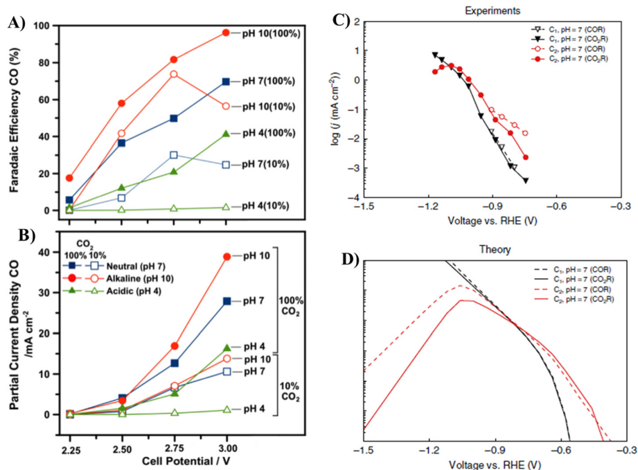
Fig. 15 (A) Faradaic efficiency for CO and (B) partial current density of CO as a function of cell potential for 3 different pH levels and two different \text{CO}_2 concentrations (10 and 100%). Comparison of ECR of \text{CO}_2 and CO at pH 7: (C) measured CO and \text{CO}_2 reduction activities toward \text{C}_1 and \text{C}_2 at pH = 7 and (D) theoretically predicted polarization curves of ECR of \text{CO}_2 and CO on Cu(211) at pH = 7. 197
