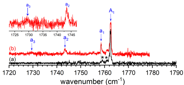
Fig. 2 Mass-selected ( m/z = 53 ) IR spectra in the \text{C}=\text{O} stretching region of (a) the PA monomer ( p_{\text{PA}} = 3 \times 10^{-5} mbar) and (b) the \text{PA} \cdots \text{D}_2\text{O} complex via a sequential pickup of PA ( p_{\text{PA}} = 3 \times 10^{-5} mbar) and \text{D}_2\text{O} ( p_{\text{D}_2\text{O}} = 3 \times 10^{-5} mbar) in helium nanodroplets. IR absorption bands of PA and the \text{PA} \cdots \text{D}_2\text{O} complex are denoted by A_1 and a_1 – a_3 , respectively. In the inset, we plot the range 1725 – 1750 \text{ cm}^{-1} displaying the bands a_2 and a_3 . The substantially weak features in trace 2a are marked with asterisks.
