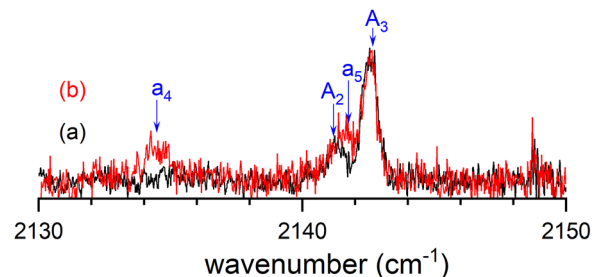
Fig. 3 Mass-selected ( m/z = 53 ) IR spectra in the \text{C}\equiv\text{C} stretching region of (a) PA monomer ( p_{\text{PA}} = 3 \times 10^{-5} mbar) and (b) \text{PA} \cdots \text{D}_2\text{O} complex via a sequential pickup of PA ( p_{\text{PA}} = 3 \times 10^{-5} mbar) and \text{D}_2\text{O} ( p_{\text{D}_2\text{O}} = 3 \times 10^{-5} mbar) in helium nanodroplets. Traces a and b are normalized to the intensity of the A_3 band. The strongest IR absorption of the monomer is denoted as A_3 and the shoulder to A_2 . The bands marked with a_4 and a_5 correspond to the \text{PA} \cdots \text{D}_2\text{O} complex.
