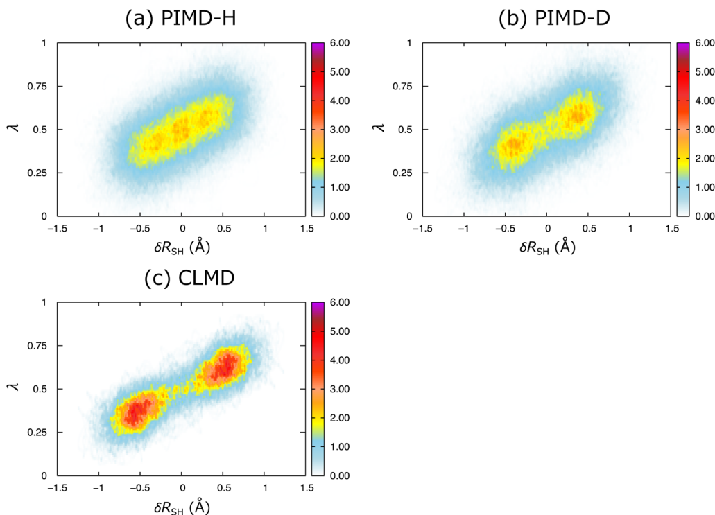
Fig. 5 Two-dimensional distributions of \delta R_{\text{SH}} and \lambda for dithiobiuret by (a) PIMD-H, (b) PIMD-D, and (c) CLMD simulations.
