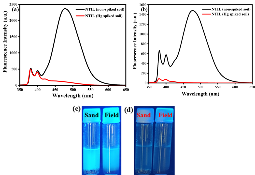
Fig. 7 (a) Variations in fluorescence intensity observed in sandy soil. (b) Variations in fluorescence intensity observed in field soil. (c) Images of nNTIL (49 \mu M) without spiking soil samples with Hg 2+ . (d) Images of nNTIL (49 \mu M) when the soil samples were spiked with Hg 2+ ions ( 10^{-2} M).
