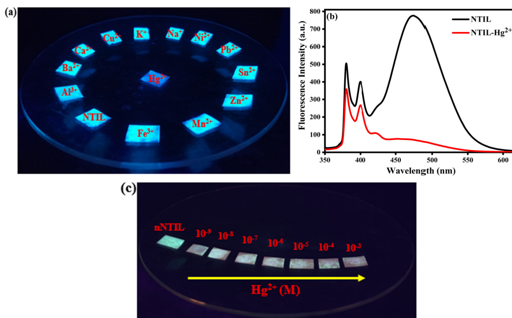
Fig. 8 (a) Images of test strips after being immersed in nNTIL (49 \mu M) alongside various metal ions ( 10^{-2} M) used in the selectivity experiment. (b) Changes in the fluorescent intensity of the paper strip with and without Hg 2+ ions ( 10^{-2} M). (c) An illustrative photograph depicting nNTIL-coated paper strips after being exposed to varying concentrations of Hg 2+ ions ( 10^{-3} – 10^{-9} M) when illuminated by a 365 nm UV lamp.
