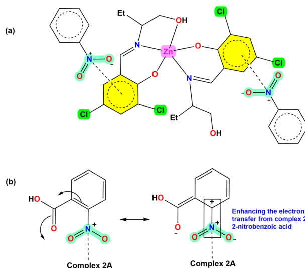
Scheme 5 (a) Schematic representation of electron transfers from complex 2A to 2-nitrobenzoic acid; (b) schematic representation of the canonical structures of 2-nitrobenzoic acid and its impact on the quenching mechanism.
