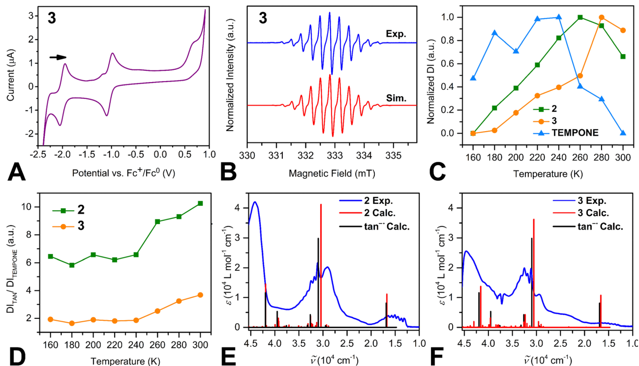
Fig. 2 (A) Cyclic voltammogram of [\text{K}(\text{crypt-222})]\text{tan}^\bullet , 3 , vs. Fc. (B) X-band cw-EPR spectrum of 3 . The experimental spectrum was collected at 300 K (blue trace) and the simulation is shown in red trace. (C) Temperature dependence of normalized EPR double intensity (DI) values of 2 (green squares), 3 (orange circles), and the standard TEMPONE (light blue triangles). (D) Corrected EPR DI values of 2 (green squares) and 3 (orange circles) obtained by dividing the DI of \text{tan}^\bullet by DI of TEMPONE at each respective temperature. UV-Vis spectra of (E) 20 \mu\text{M} solution of 2 and (F) 15 \mu\text{M} solution of 3 . Both spectra (blue trace) were collected in THF from 220 nm to 1000 nm. The red vertical lines correspond to predicted TD-DFT transitions. Black vertical lines exhibit the predicted transitions for the \text{tan}^\bullet fragment.
