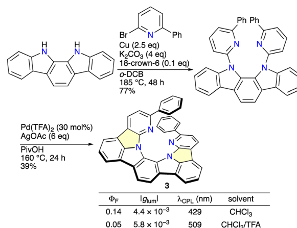
Scheme 2 Synthesis of tetraaza[7]helicene 3 .
