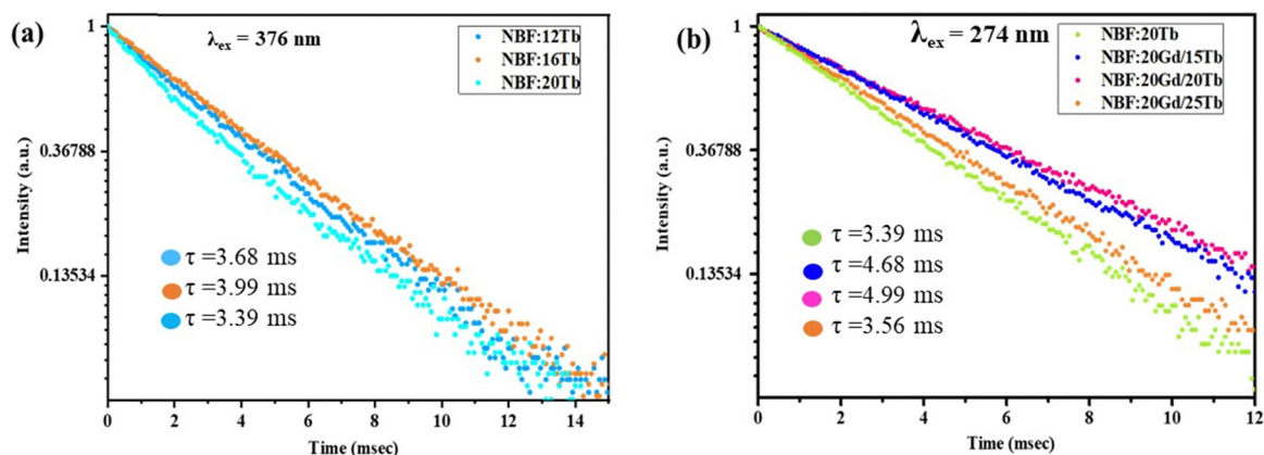
Fig. 5 (a) PL decay curves of NBF: x\text{Tb} and (b) NBF:20%Gd, x\text{Tb} ( x = 15, 20, 25 ) nanoparticles.
