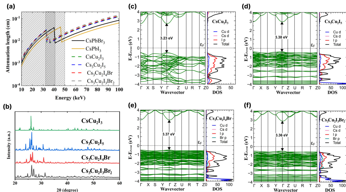
Fig. 1 (a) X-ray attenuation lengths for the investigated caesium copper perovskites (CHPs) with CsPbI 3 and CsPbBr 3 used as in ref. 4. (b) XRD spectra of the CHPs. Band structures and density of states of (c) CsCu 2 I 3 , (d) Cs 3 Cu 2 I 5 , (e) Cs 3 Cu 2 I 4 Br, and (f) Cs 3 Cu 2 I 3 Br 2 .
