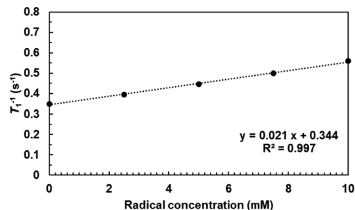
Fig. 5 Plot of T_1 relaxation rates of H 2 O protons versus the concentration of TTM-PEG3 in water.
