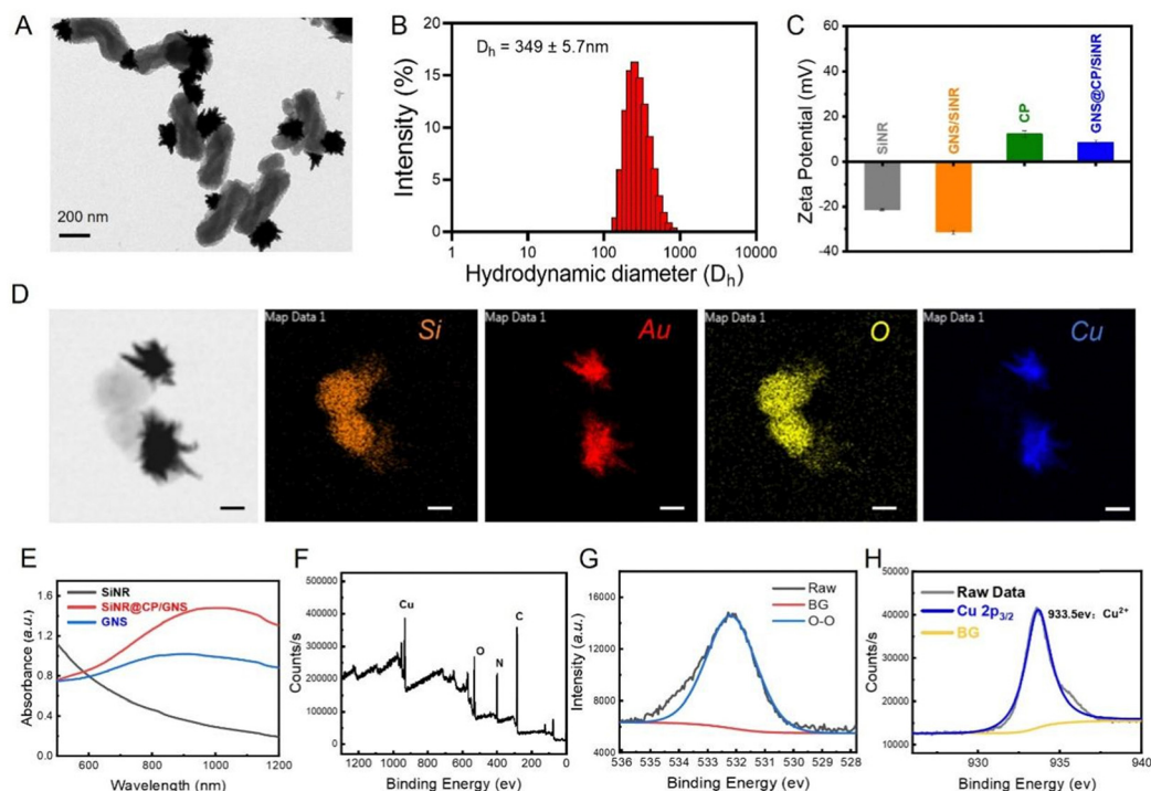
Fig. 1 Characterization of the GNS@CP/SiNR Janus nanostructure. (A) TEM image of the GNS@CP/SiNR Janus nanostructure, scale bar represents 200 nm. (B) Intensity-weighted size distribution of the GNS@CP/SiNR Janus nanostructure. (C) Zeta potentials of SiNR, GNS/SiNR, CP and the GNS@CP/SiNR Janus nanostructure. (D) Elemental mapping image of GNS@CP/SiNR. (E) UV-Vis-NIR spectra of SiNR, GNS and SiNR@CP/GNS. (F) Survey XPS spectrum of GNS@CP/SiNR and high-resolution XPS spectra of O 1s (G) and Cu 2p (H).
