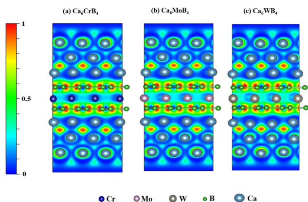
Fig. 4 Electron localization functions (ELFs) of the (100) section on (a) Ca 6 CrB 4 , (b) Ca 6 MoB 4 , and (c) Ca 6 WB 4 .
