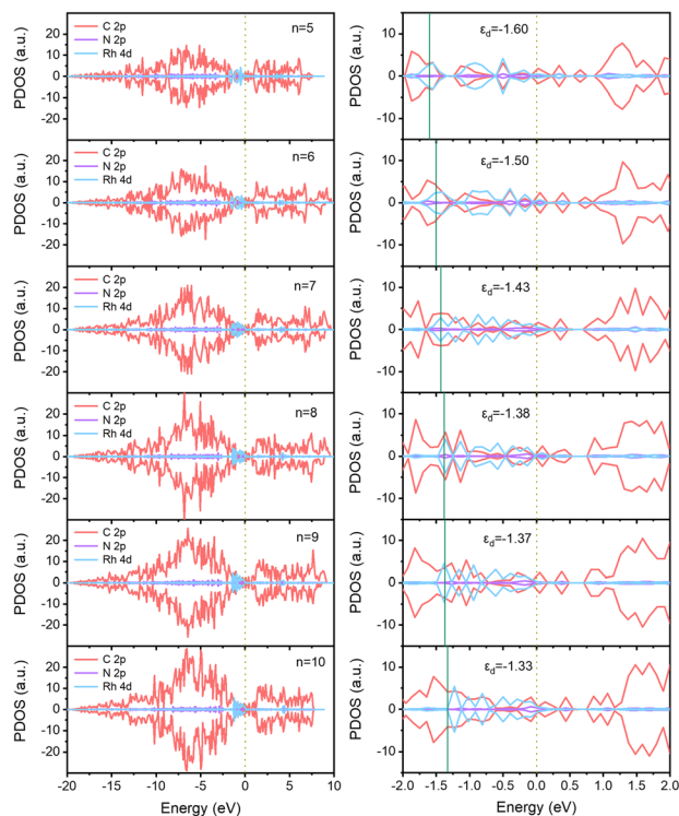
Fig. 4 Partial density of states (PDOS) for \text{RhN}_4@\text{CNTs}(n, n) ( n = 5-10 ). C-state, N-state, and Rh-state are represented by red, purple, and blue. On the right is an enlarged view in the energy range of -2 to 2 eV. The dotted line and the full line represent the position of the Fermi level and d-band center ( \epsilon_d ), respectively.
