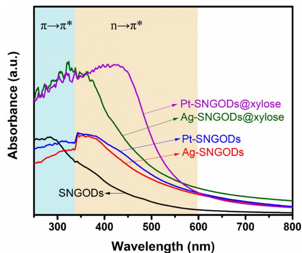
Fig. 1 Optical absorption spectra of the aqueous suspensions of SNGODs, Pt-SNGODs, Ag-SNGODs, Pt-SNGODs@xylose, and Ag-SNGODs@xylose. The absorption was arisen from the \pi \rightarrow \pi^* and n \rightarrow \pi^* transitions.
