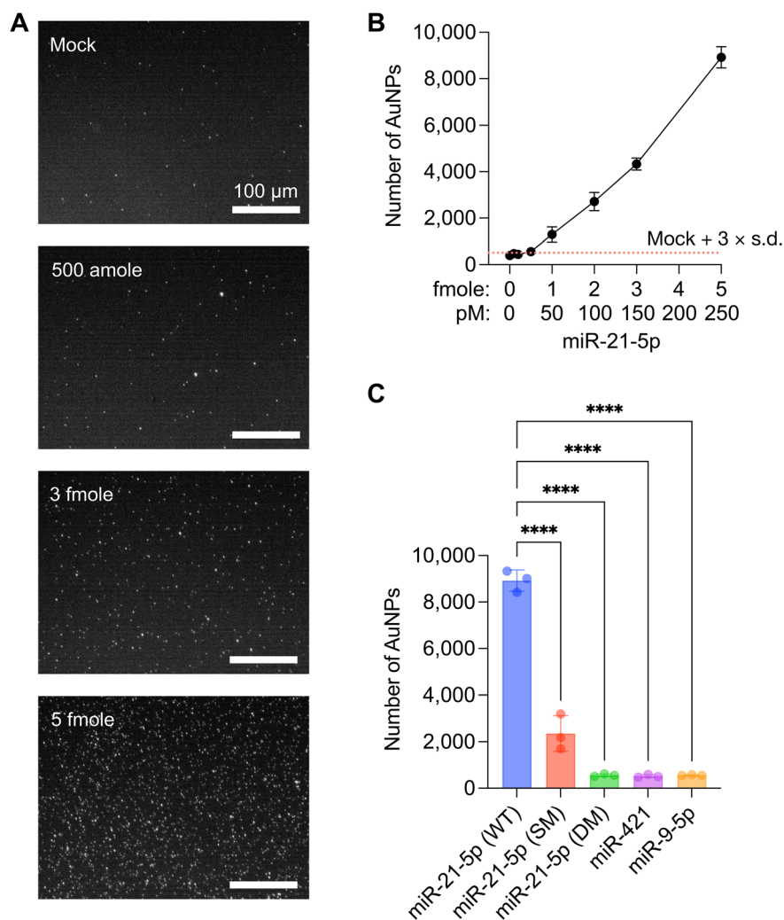
Fig. 3 Evaluation of sensitivity and specificity of the CRISPR/Cas13a-assisted MGNP-DF assay. A and B . Measurement of released AuNPs by seven different concentrations of miR-21-5p. A . Representative zoomed-in images for the 4 different target miRNA amounts. Scale bar, 100 \mu m. B . Quantitative analysis for the numbers of released AuNPs. The dotted line indicates the number of mean + 3 \times standard deviation (s.d.) of the mock sample. Error bars are shown as mean \pm s.d. from three independent experiments. C . Detection specificity was evaluated using wildtype (WT), single-mismatch (SM), and double-mismatches (DM) of miR-21-5p, miR-421, and miR-9-5p. Bar graphs are shown as mean \pm SD from the three experiments. **** P < 0.0001 compared miR-21-5p (WT) sample, as assessed by two-way ANOVA with Bonferroni's multiple comparisons test.
