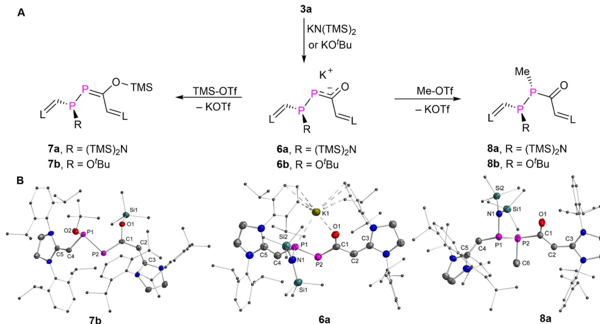
Fig. 5 (A) Synthesis of 6 – 8 . (B) Plots of the molecular structure of 6a , 7b , and 8a (ellipsoids are set to 50% probability; H atoms and solvents are omitted for clarity). Selected distances (Å): 6a : P1–K1 3.1275(6), O1–K1 2.5557(11), P1–N1 1.7716(13), P1–P2 2.1923(6), P2–C1 1.8058(17), C1–O1 1.2705(19), C1–C2 1.469(2), C2–C3 1.360(2), P1–C4 1.7957(17), C4–C5 1.352(2); 7b : P1–O2 1.6834(13), O1–Si1 1.6593(13), P1–P2 2.2243(7), P2–C1 1.7203(19), C1–O1 1.390(2), C1–C2 1.430(3), C2–C3 1.370(3), P1–C4 1.7903(19), C4–C5 1.353(3); 8a : P1–N1 1.739(3), P2–C6 1.862(3), P1–P2 2.2367(10), P2–C1 1.891(3), C1–O1 1.229(4), C1–C2 1.424(4), C2–C3 1.384(4), P1–C4 1.797(3), C4–C5 1.363(4).
