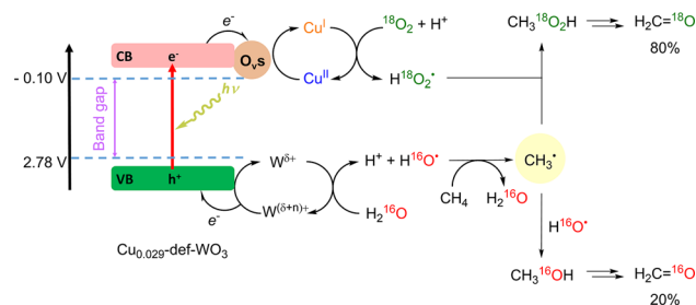
Fig. 21 Proposed mechanism for charge transfer steps during selective \text{CH}_4 oxidation over \text{Cu}_{0.029}\text{-def-WO}_3 .
