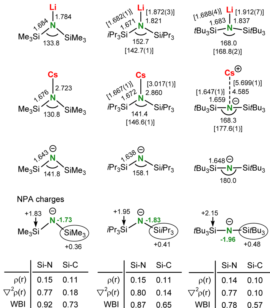
Scheme 5 Comparison of DFT-optimized Li and Cs amide complexes and the free anions \text{MeN}^- , i\text{PrN}^- and t\text{BuN}^- (B3PW91/def2tzvp including GD3BJ dispersion corrections) showing distances (Å), angles (°), Wiberg bond indices (WBIs) and values for \rho(r) and the Laplacian \nabla^2\rho(r) in the bond-critical point (a.u.). Values for crystal structures are given between square brackets.
