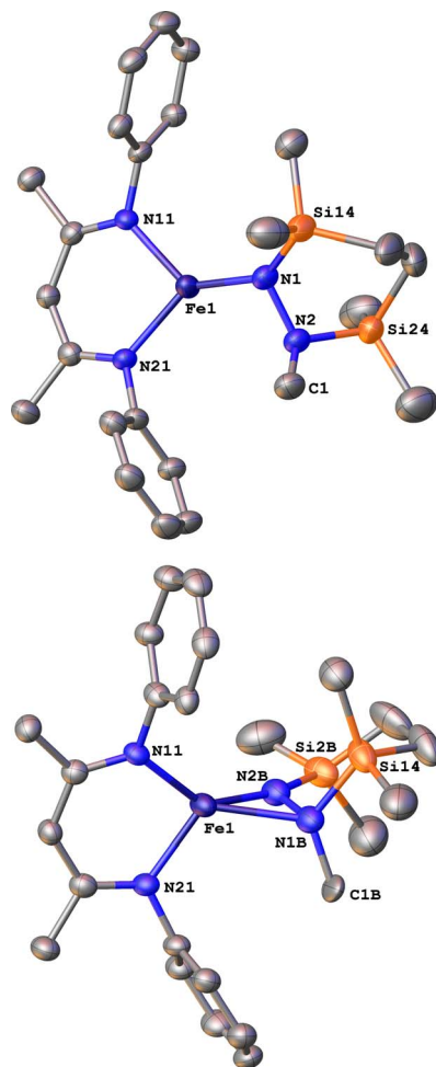
Fig. 7 ORTEP diagrams of 10-1 and 10-2 with thermal ellipsoids shown at 50% probability and H atoms and 1 Pr groups omitted for clarity. The \eta^1 isomer (major component 10-1, 75%) is shown on the top, and the \eta^2 isomer (minor component 10-2, 25%) is shown on the bottom.
