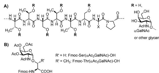
Fig. 1 (A) Tandem repeat motif (TTSTTSPX) for MUC5AC. (B) Fmoc-Ser/Thr( \alpha Ac 3 GalNAc)-OH building blocks.
