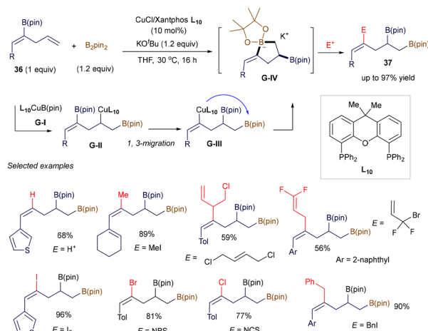
Scheme 11 Boron-copper 1,3-rearrangement.
