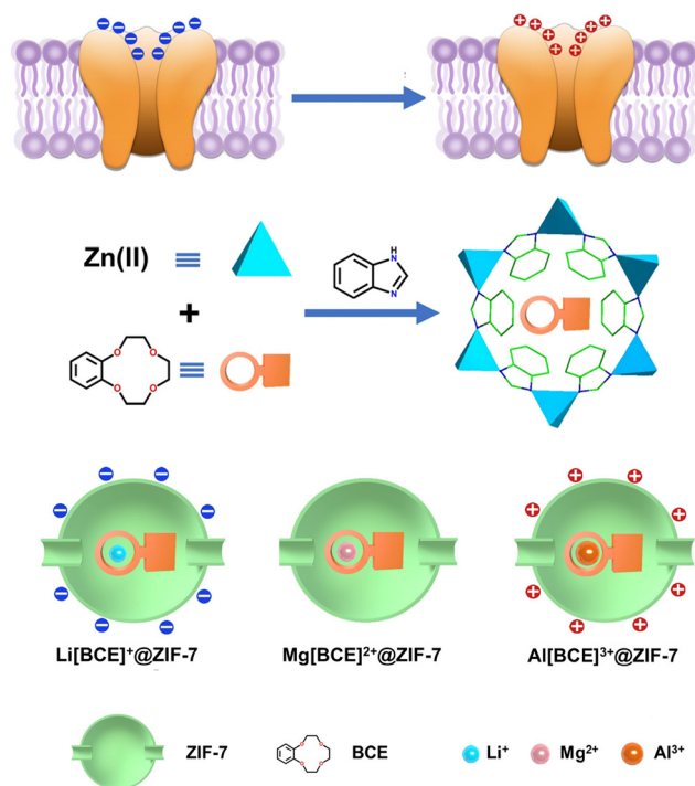
Fig. 2 Scheme illustration for the construction of M[BCE] n+ @ZIF-7 (M = Li + , Mg 2+ , Al 3+ ). 66 Copyright 2023 Wiley-VCH.
